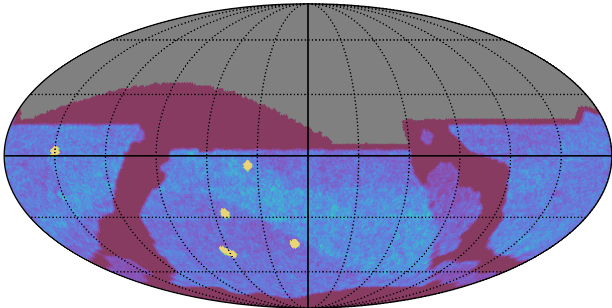
internal_u_expt38_nscale1.0v3.4_10yrs All sky z band: NVisits
