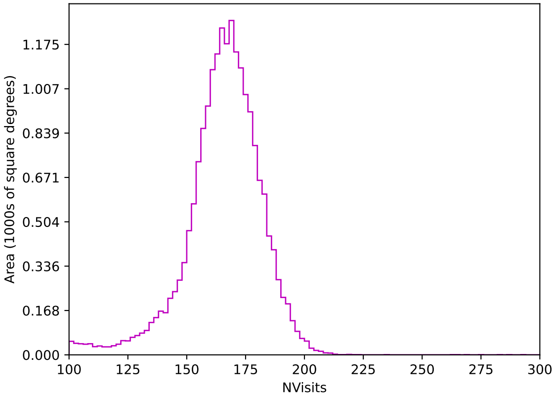
internal_u_expt38_nscale1.0v3.4_10yrs All sky z band: NVisits
