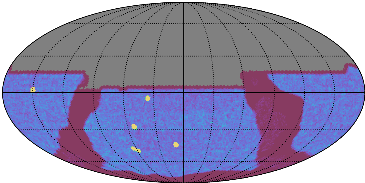
internal_u_expt38_nscale1.0v3.4_10yrs All sky y band: NVisits
