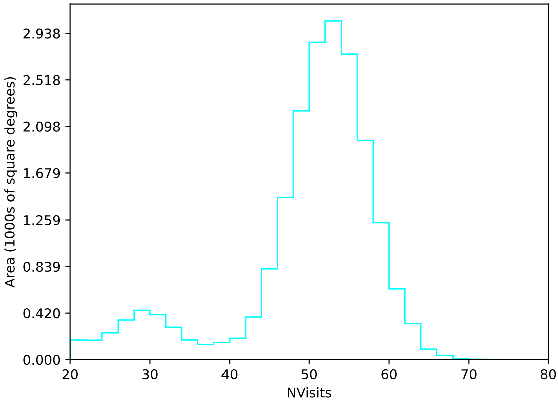
internal_u_expt38_nscale1.0v3.4_10yrs All sky u band: NVisits
