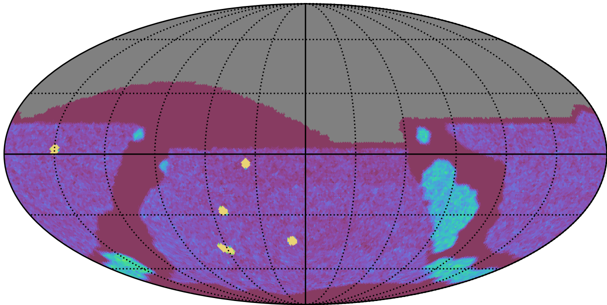
internal_u_expt38_nscale1.0v3.4_10yrs All sky g band: NVisits
