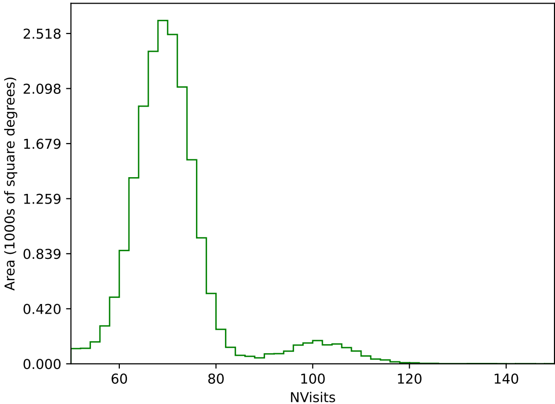
internal_u_expt38_nscale1.0v3.4_10yrs All sky g band: NVisits
