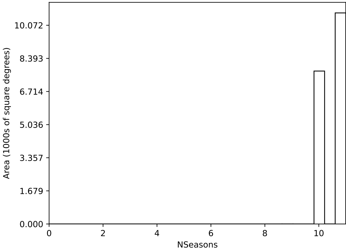
internal_u_expt38_nscale1.0v3.4_10yrs WFD all bands: NSeasons
