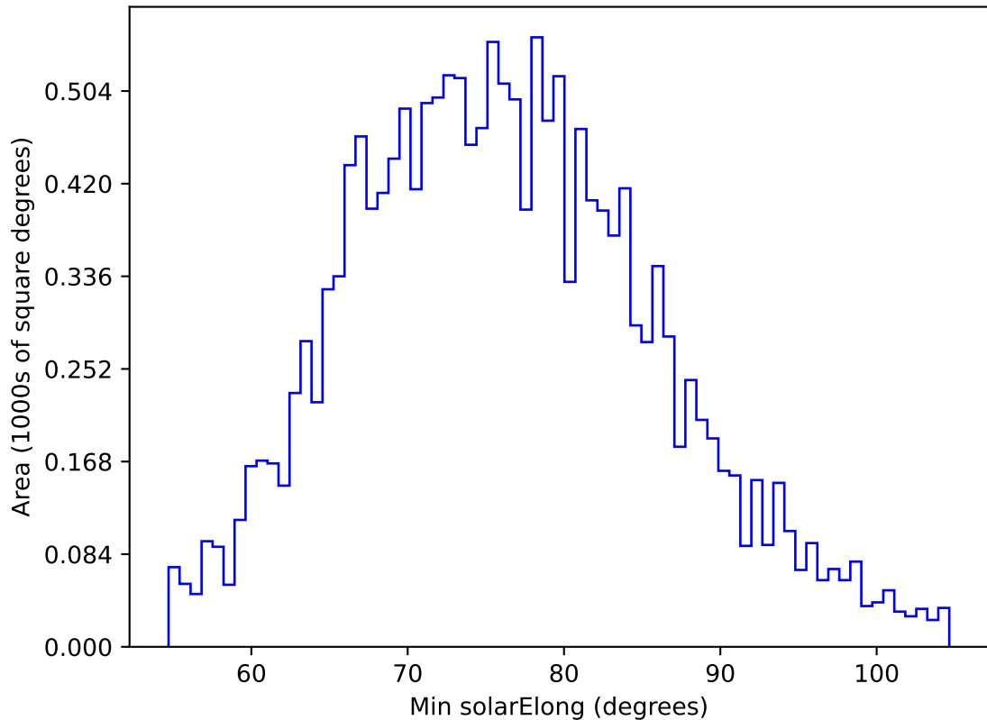
internal_u_expt38_nscale1.0v3.4_10yrs WFD g band: Min solarElong
