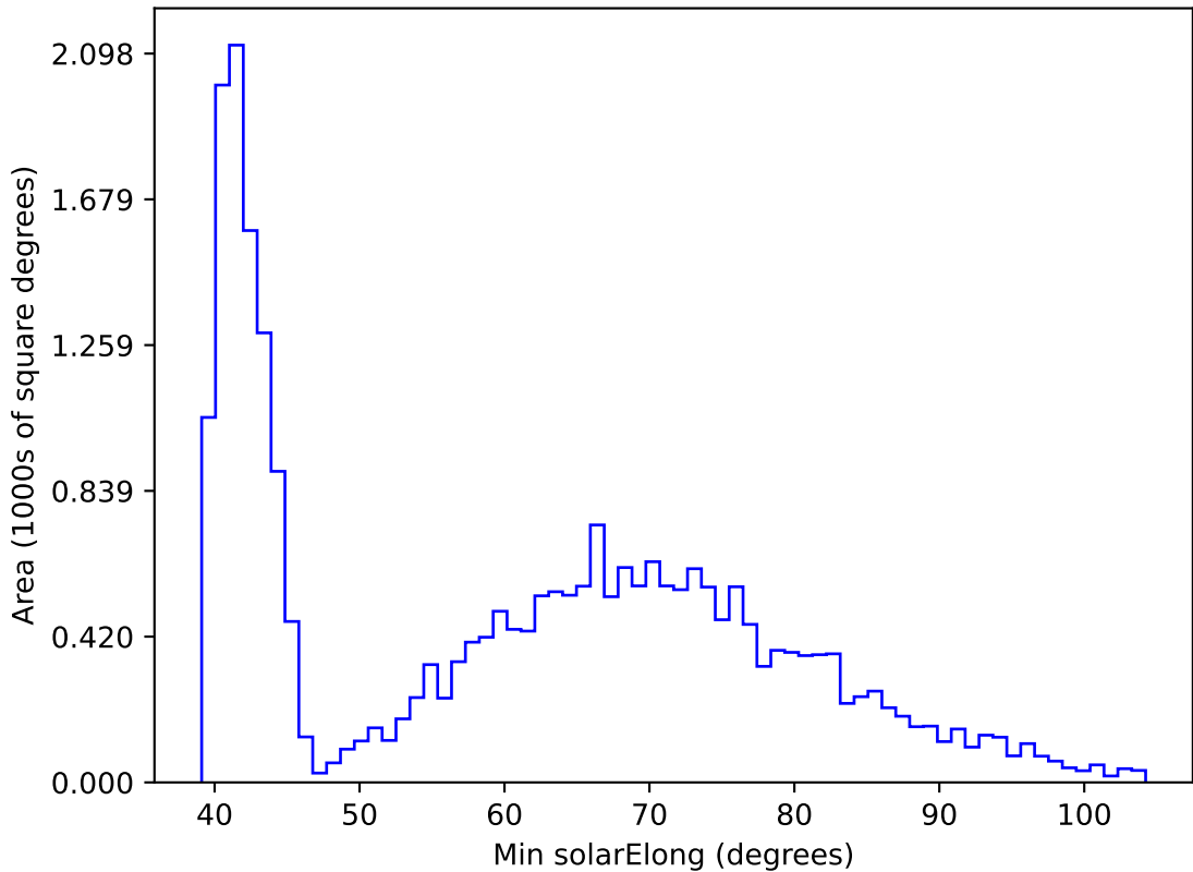
internal_u_expt38_nscale1.0v3.4_10yrs All sky r band: Min solarElong
