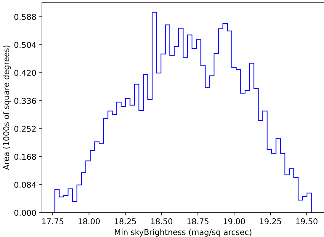
internal_u_expt38_nscale1.0v3.4_10yrs WFD r band: Min skyBrightness
