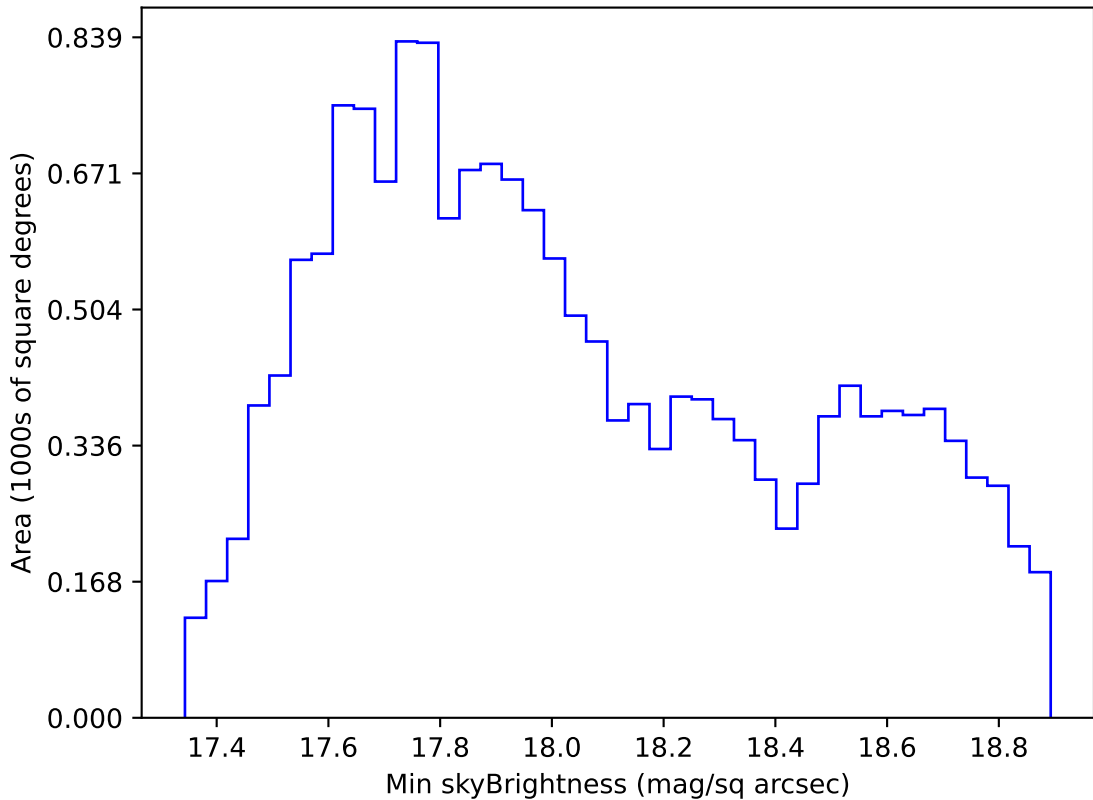
internal_u_expt38_nscale1.0v3.4_10yrs WFD i band: Min skyBrightness
