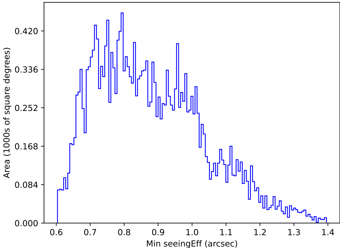
internal_u_expt38_nscale1.0v3.4_10yrs Yr 1 u band: Min seeingEff
