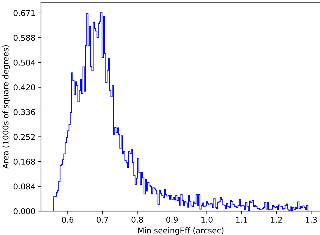
internal_u_expt38_nscale1.0v3.4_10yrs Yr 1 r band: Min seeingEff
