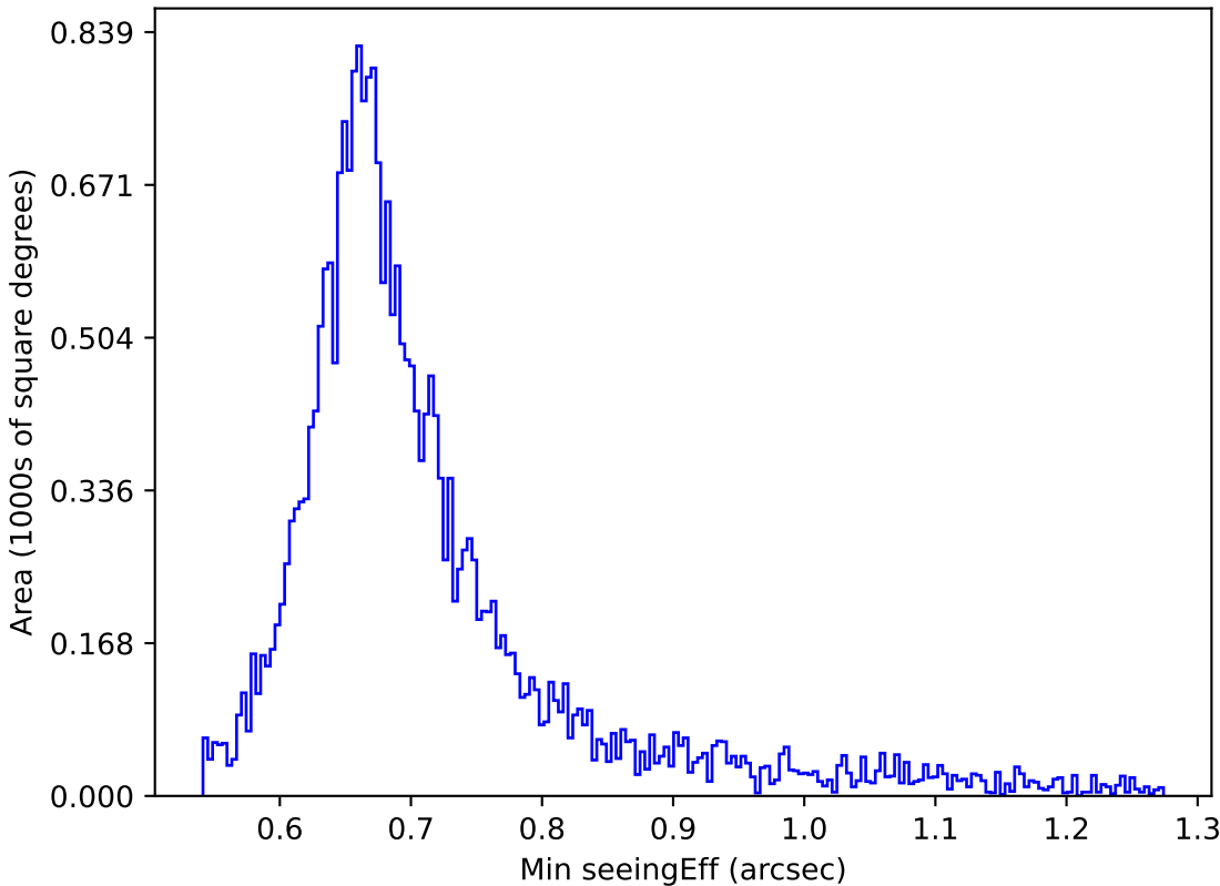
internal_u_expt38_nscale1.0v3.4_10yrs Yr 1 i band: Min seeingEff
