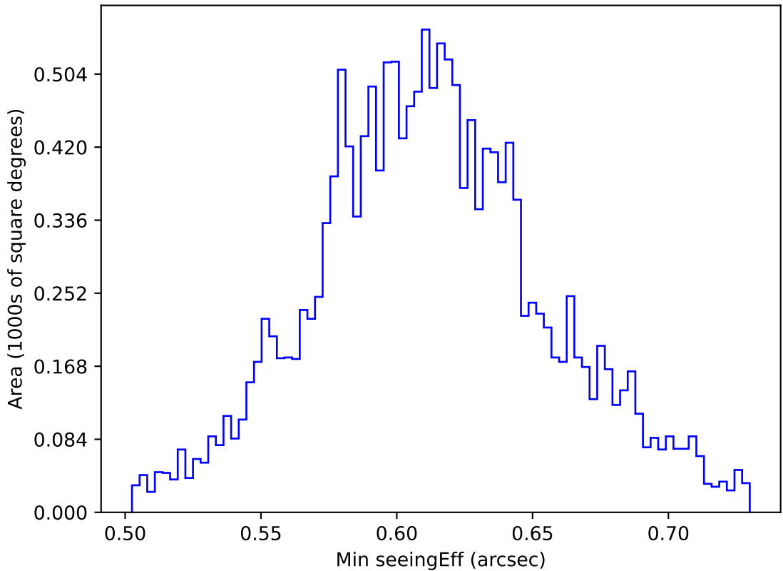
internal_u_expt38_nscale1.0v3.4_10yrs WFD z band: Min seeingEff
