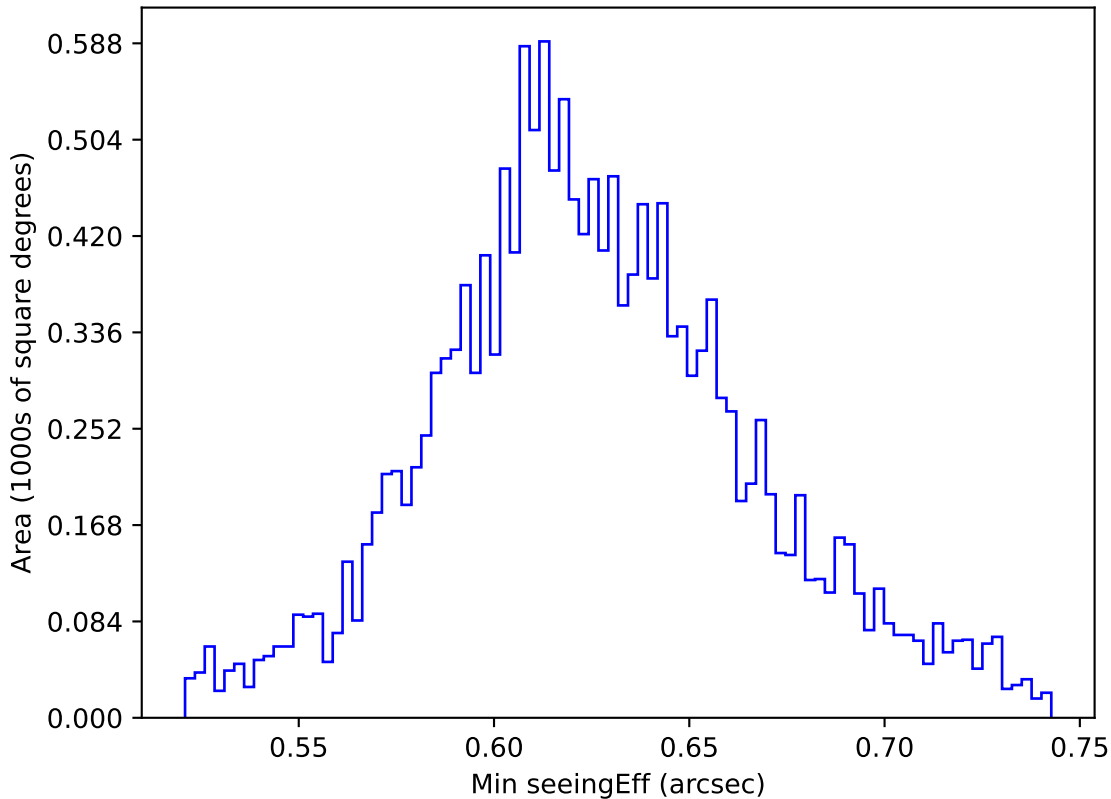
internal_u_expt38_nscale1.0v3.4_10yrs WFD y band: Min seeingEff
