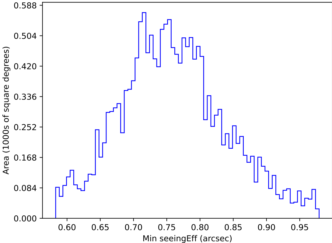
internal_u_expt38_nscale1.0v3.4_10yrs WFD u band: Min seeingEff
