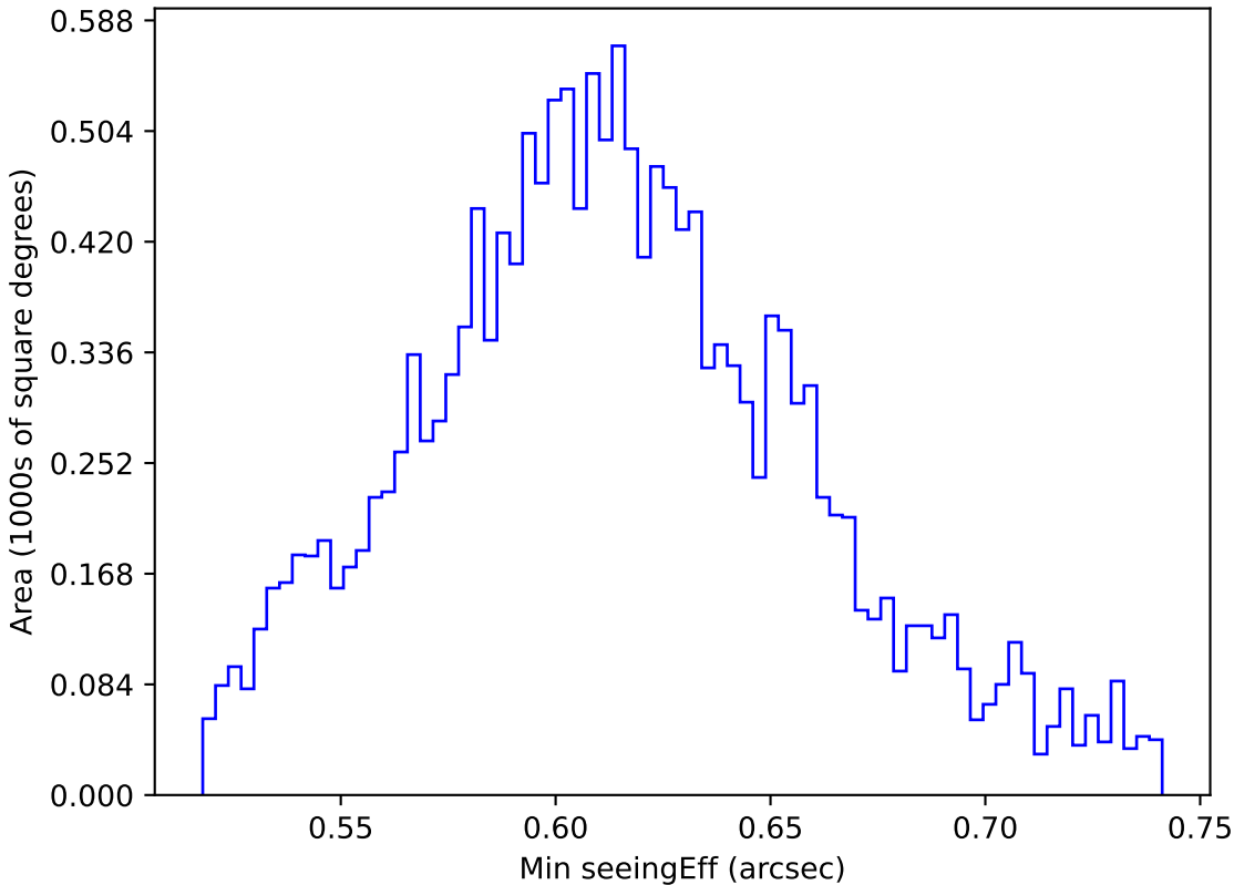
internal_u_expt38_nscale1.0v3.4_10yrs WFD r band: Min seeingEff
