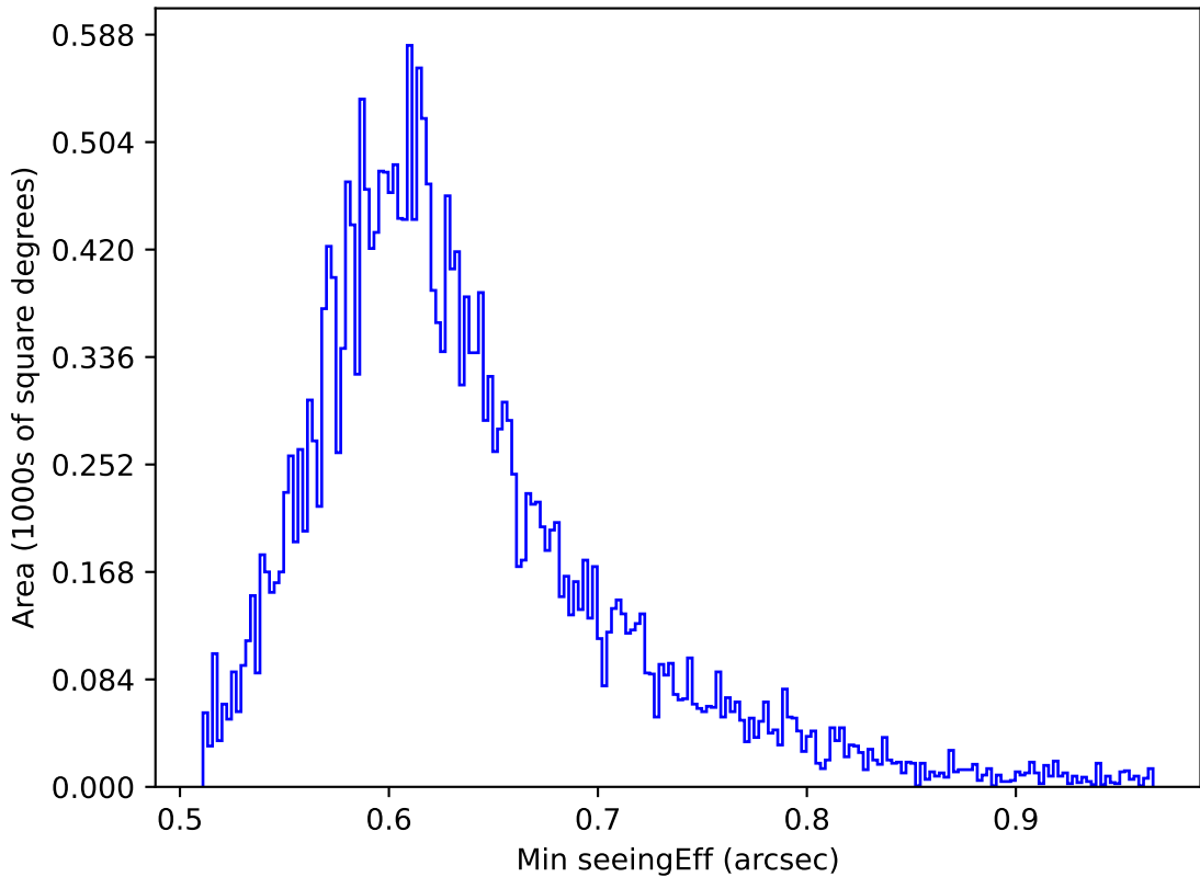
internal_u_expt38_nscale1.0v3.4_10yrs All sky i band: Min seeingEff
