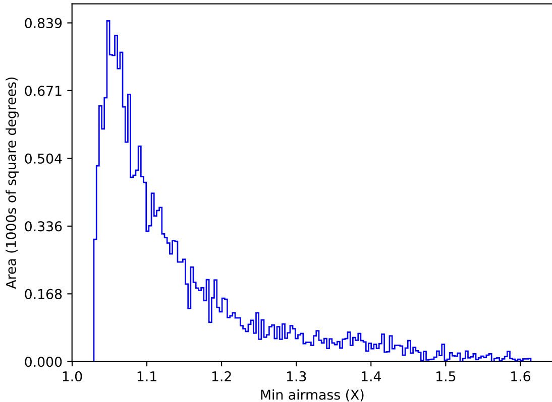
internal_u_expt38_nscale1.0v3.4_10yrs Yr 1 u band: Min airmass
