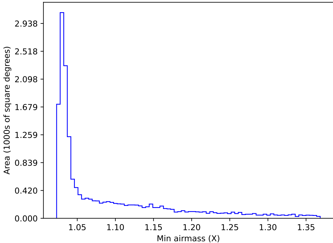
internal_u_expt38_nscale1.0v3.4_10yrs WFD y band: Min airmass
