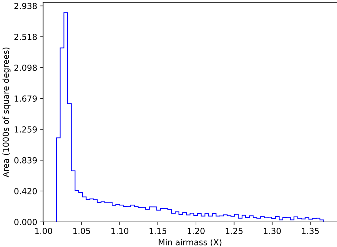
internal_u_expt38_nscale1.0v3.4_10yrs WFD r band: Min airmass
