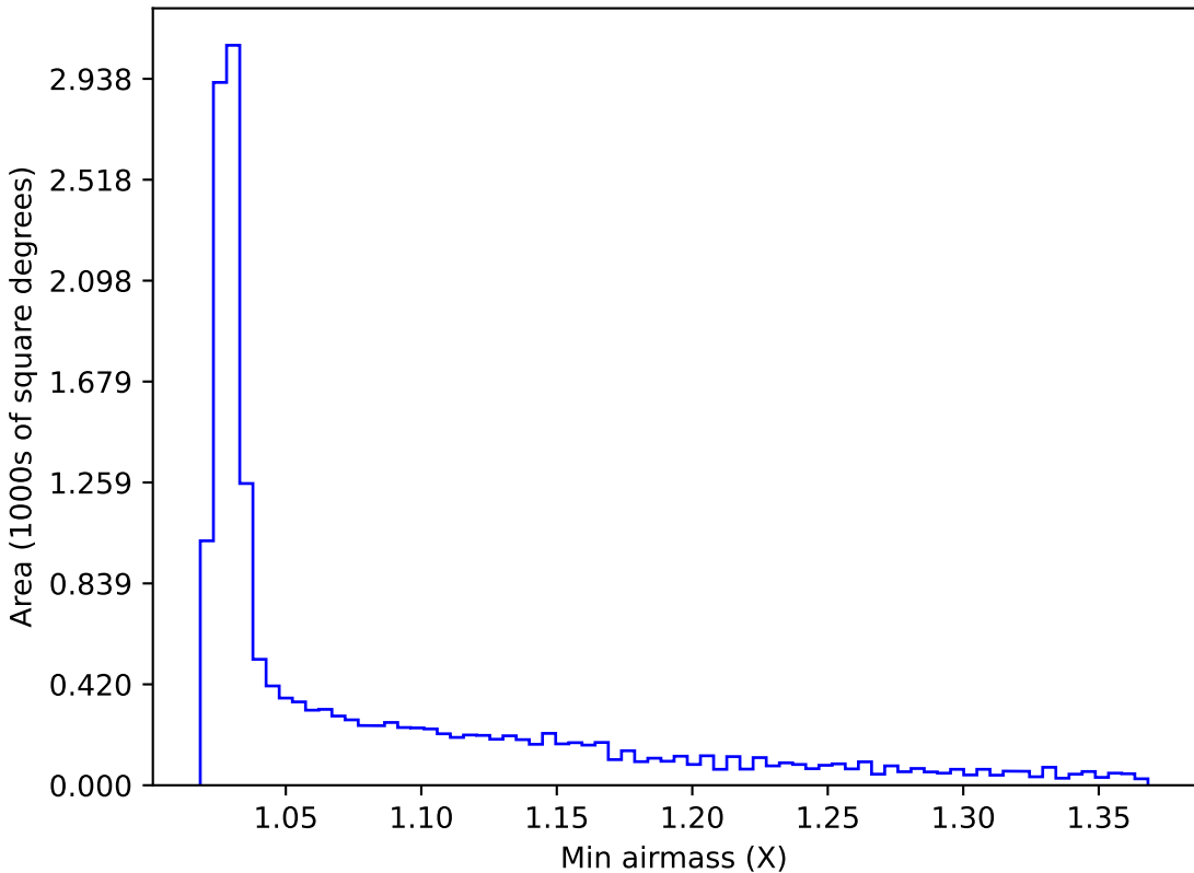
internal_u_expt38_nscale1.0v3.4_10yrs WFD i band: Min airmass
