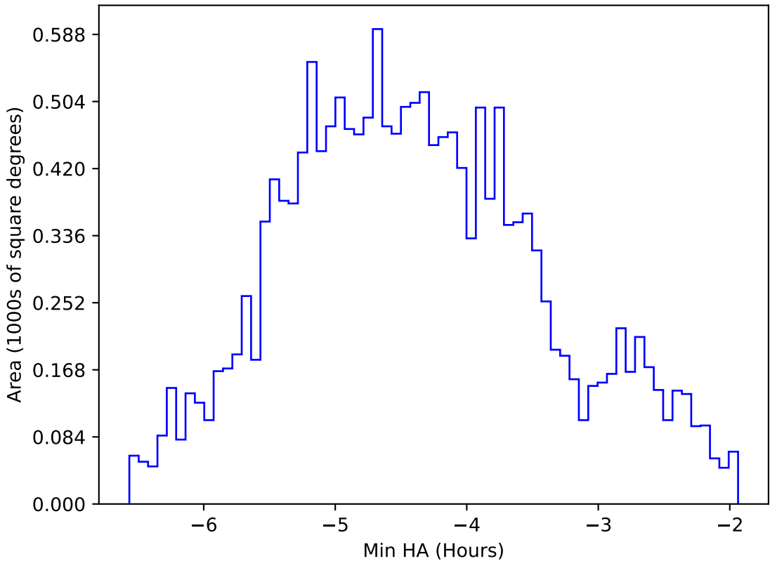
internal_u_expt38_nscale1.0v3.4_10yrs WFD z band: Min HA
