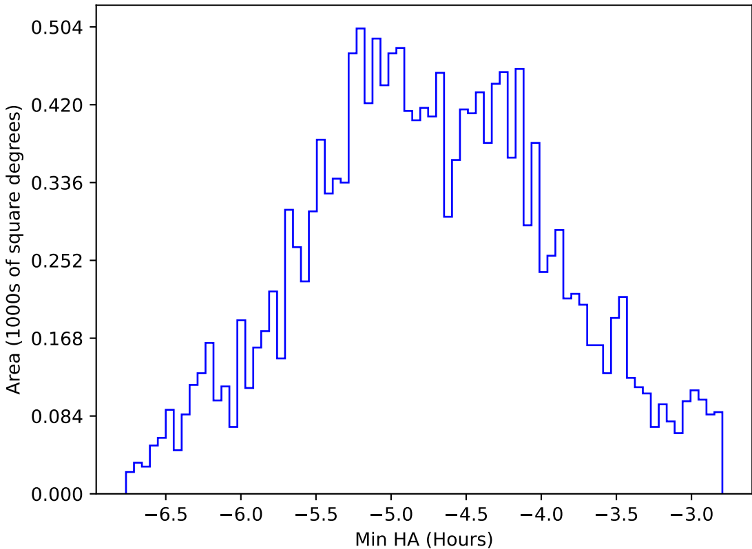
internal_u_expt38_nscale1.0v3.4_10yrs WFD all bands: Min HA
