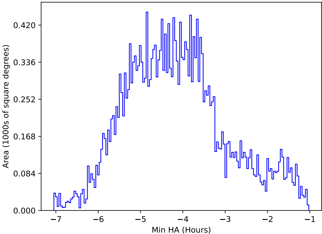
internal_u_expt38_nscale1.0v3.4_10yrs All sky r band: Min HA
