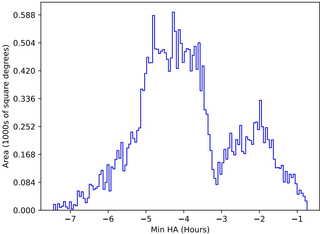
internal_u_expt38_nscale1.0v3.4_10yrs All sky g band: Min HA
