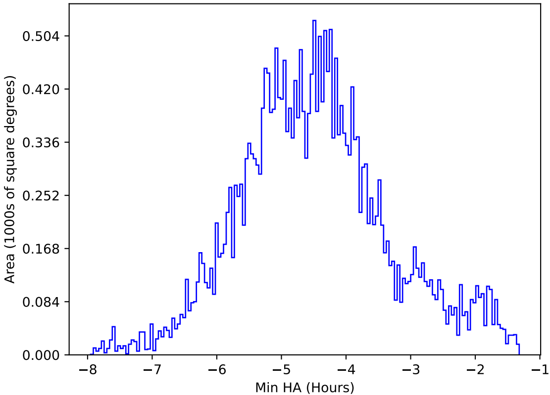
internal_u_expt38_nscale1.0v3.4_10yrs All sky all bands: Min HA
