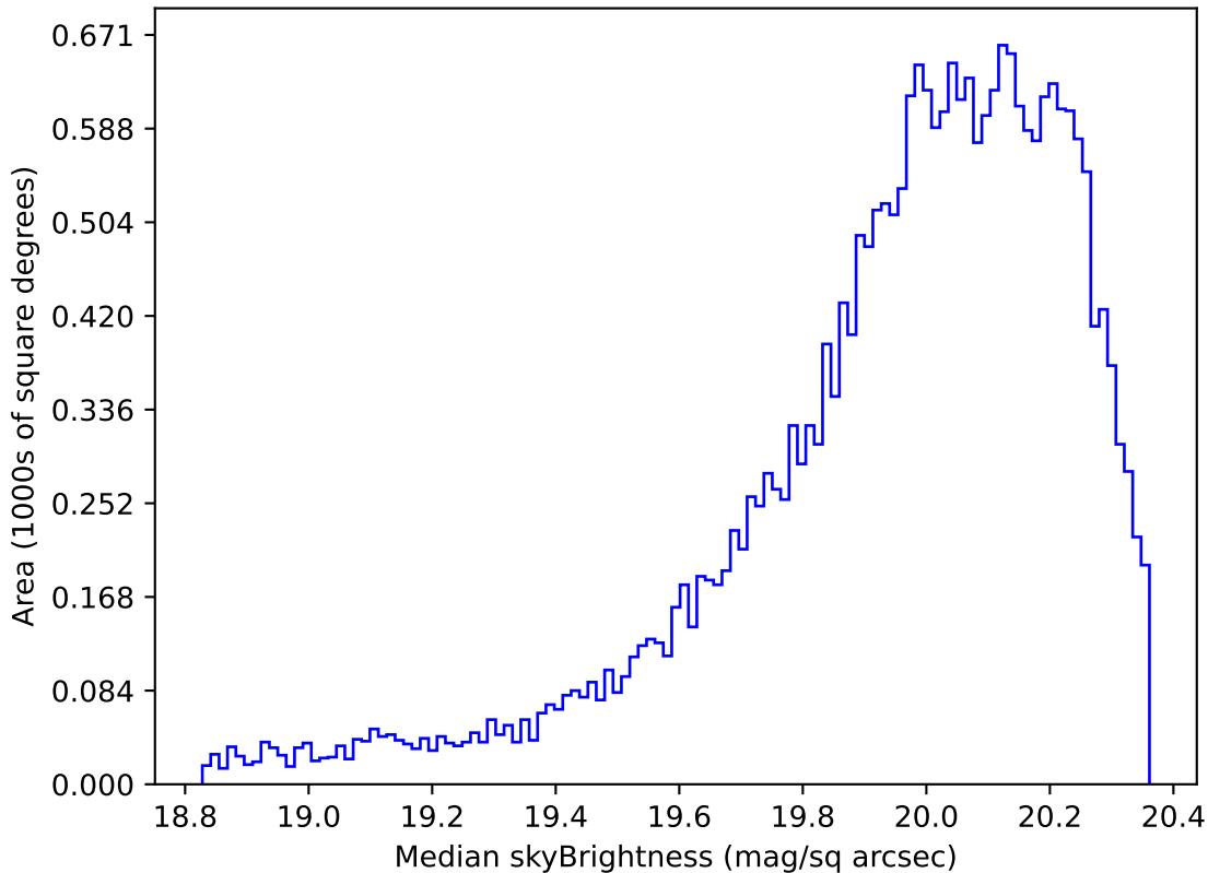
internal_u_expt38_nscale1.0v3.4_10yrs Yr 1 i band: Median skyBrightness
