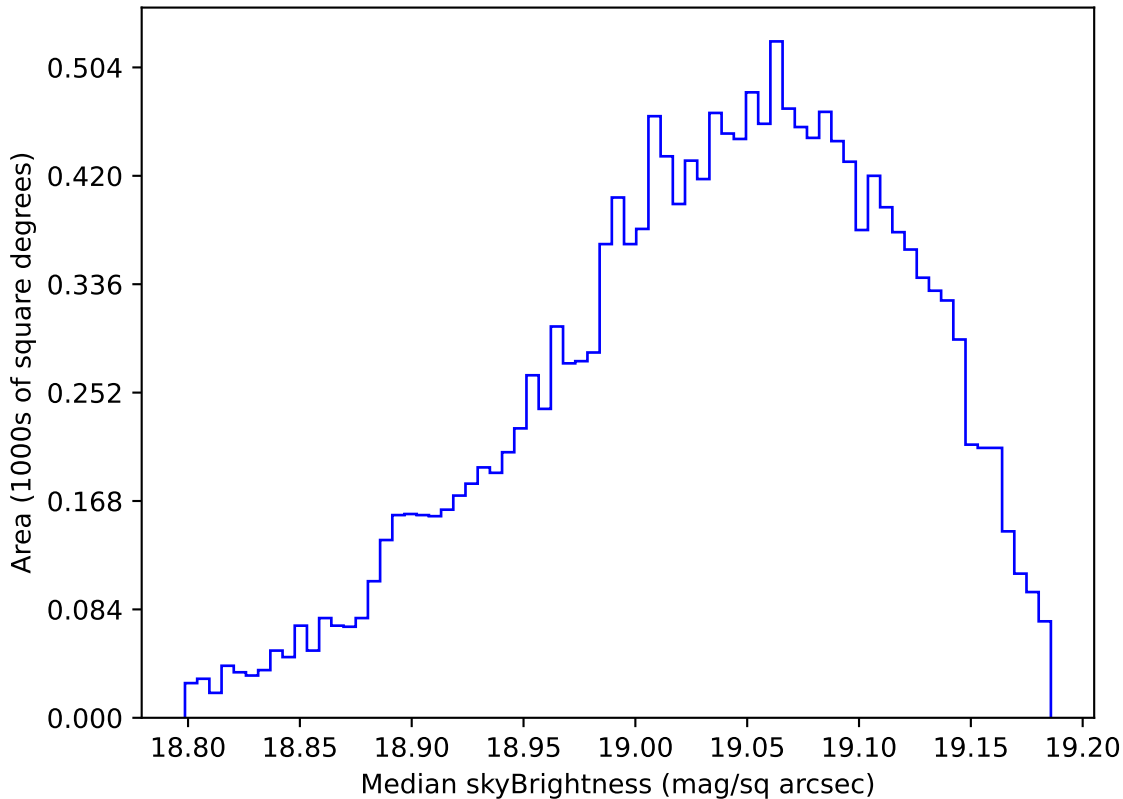
internal_u_expt38_nscale1.0v3.4_10yrs WFD z band: Median skyBrightness
