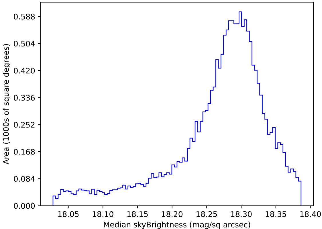
internal_u_expt38_nscale1.0v3.4_10yrs WFD y band: Median skyBrightness
