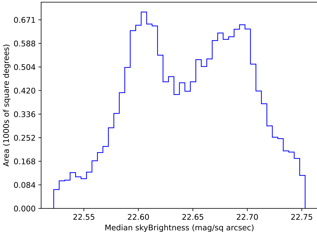
internal_u_expt38_nscale1.0v3.4_10yrs WFD u band: Median skyBrightness
