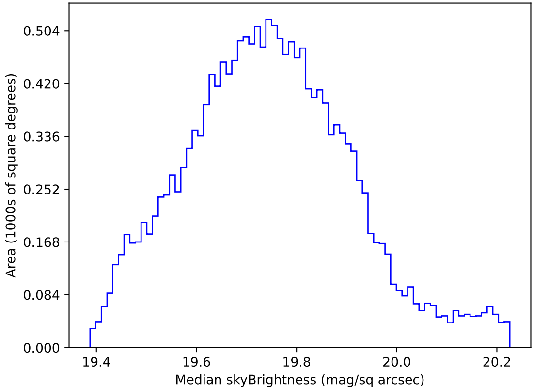
internal_u_expt38_nscale1.0v3.4_10yrs WFD all bands: Median skyBrightness
