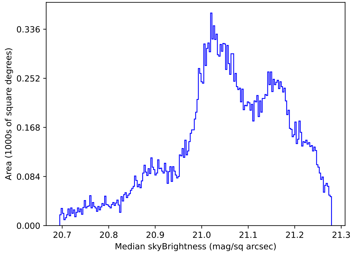
internal_u_expt38_nscale1.0v3.4_10yrs All sky r band: Median skyBrightness
