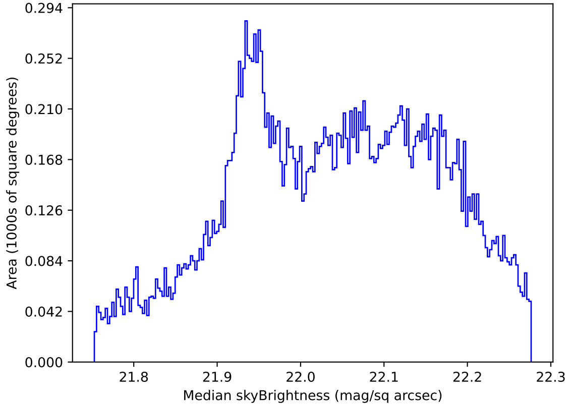
internal_u_expt38_nscale1.0v3.4_10yrs All sky g band: Median skyBrightness
