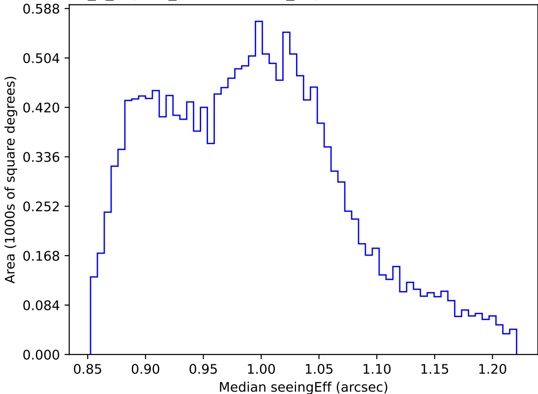
internal_u_expt38_nscale1.0v3.4_10yrs WFD i band: Median seeingEff
