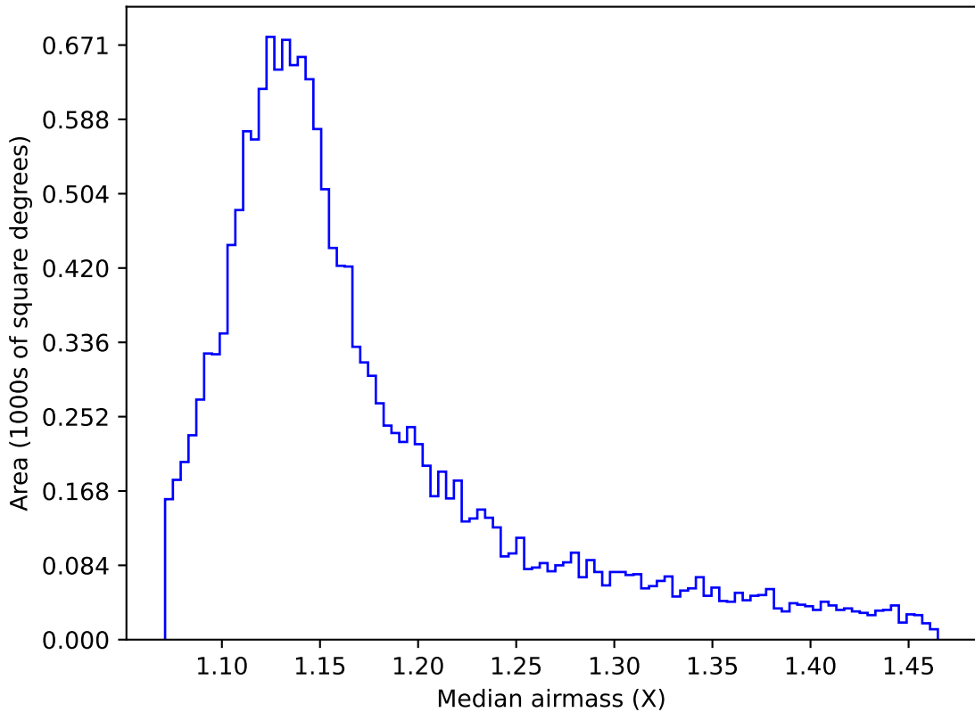
internal_u_expt38_nscale1.0v3.4_10yrs WFD u band: Median airmass
