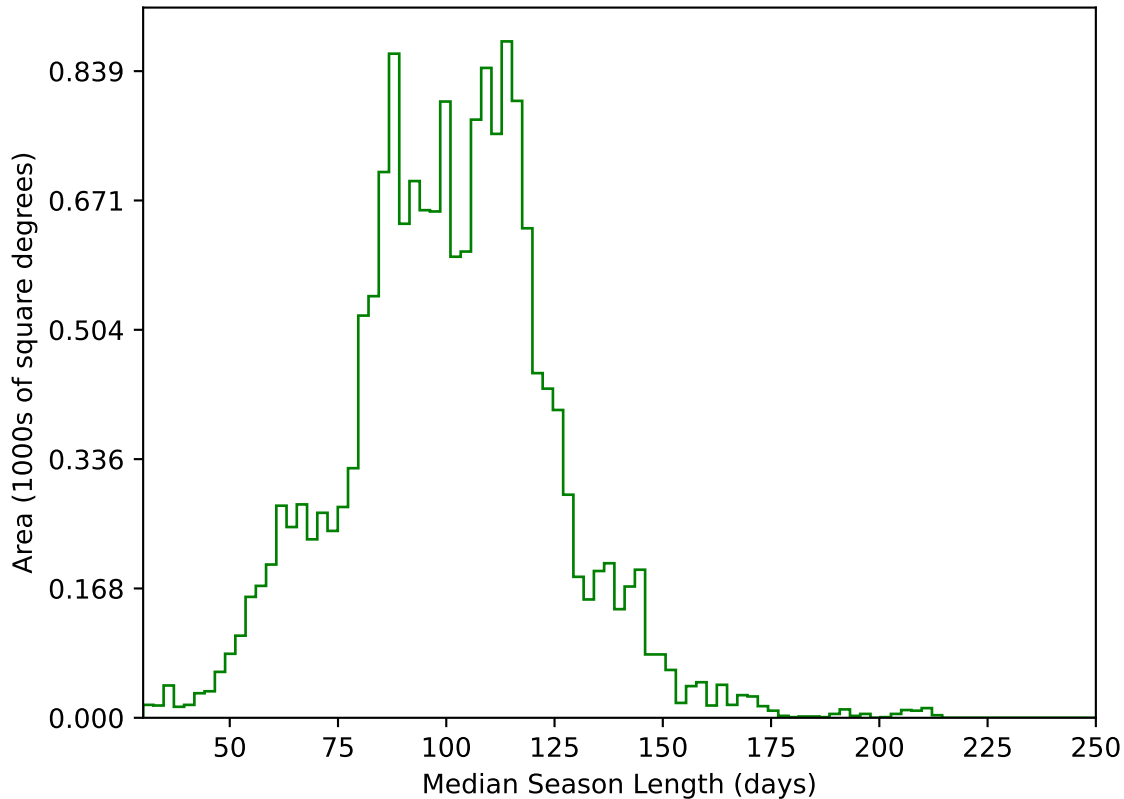
internal_u_expt38_nscale1.0v3.4_10yrs WFD g band: Median Season Length
