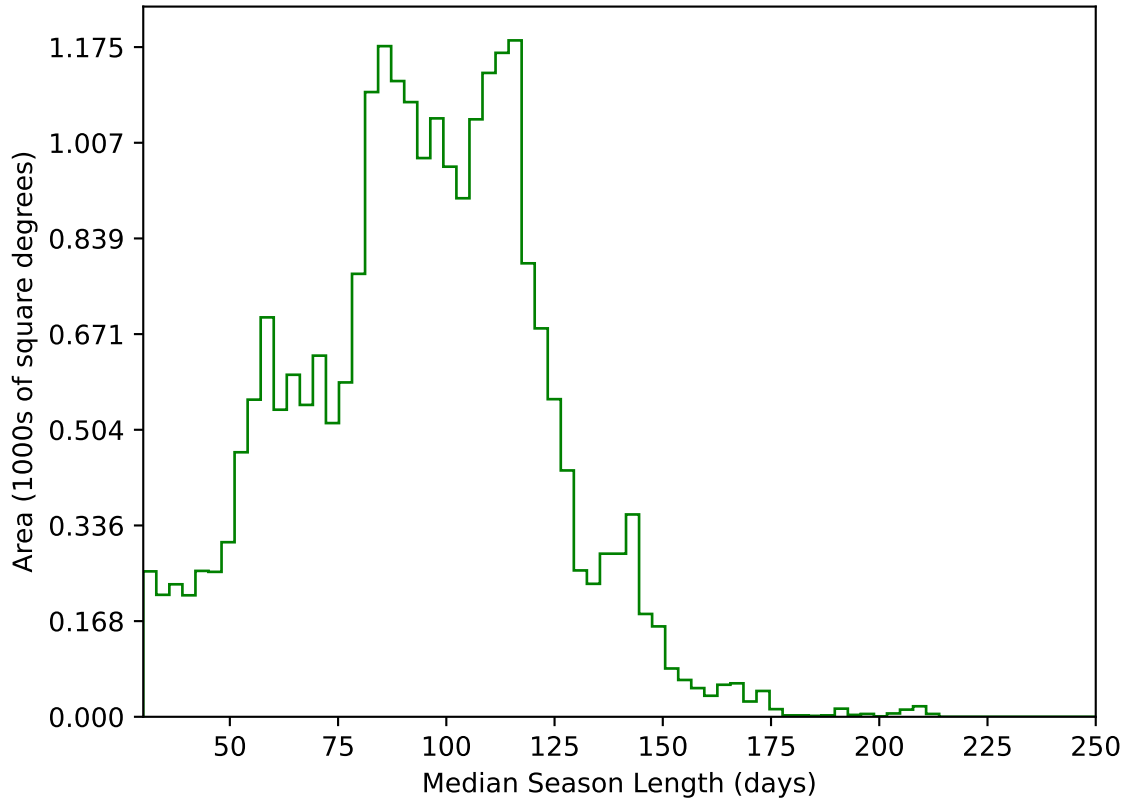
internal_u_expt38_nscale1.0v3.4_10yrs All sky g band: Median Season Length
