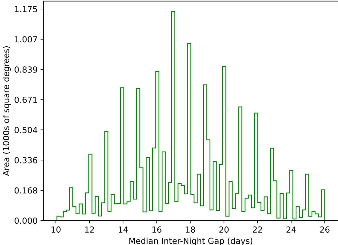
internal_u_expt38_nscale1.0v3.4_10yrs WFD g band: Median Inter-Night Gap
