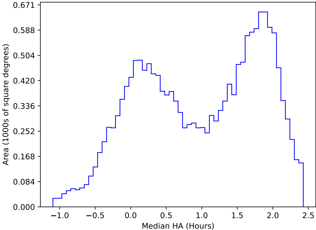
internal_u_expt38_nscale1.0v3.4_10yrs WFD u band: Median HA
