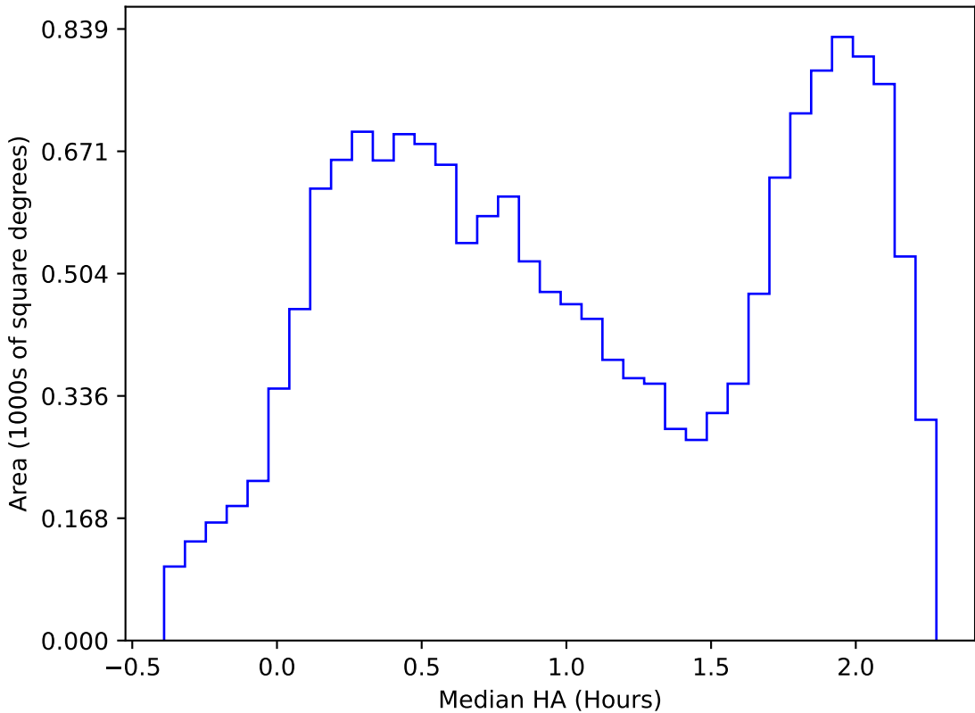
internal_u_expt38_nscale1.0v3.4_10yrs WFD i band: Median HA
