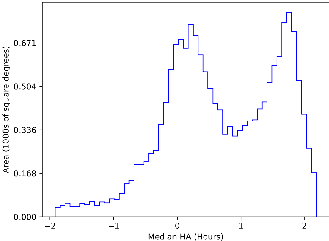
internal_u_expt38_nscale1.0v3.4_10yrs WFD g band: Median HA
