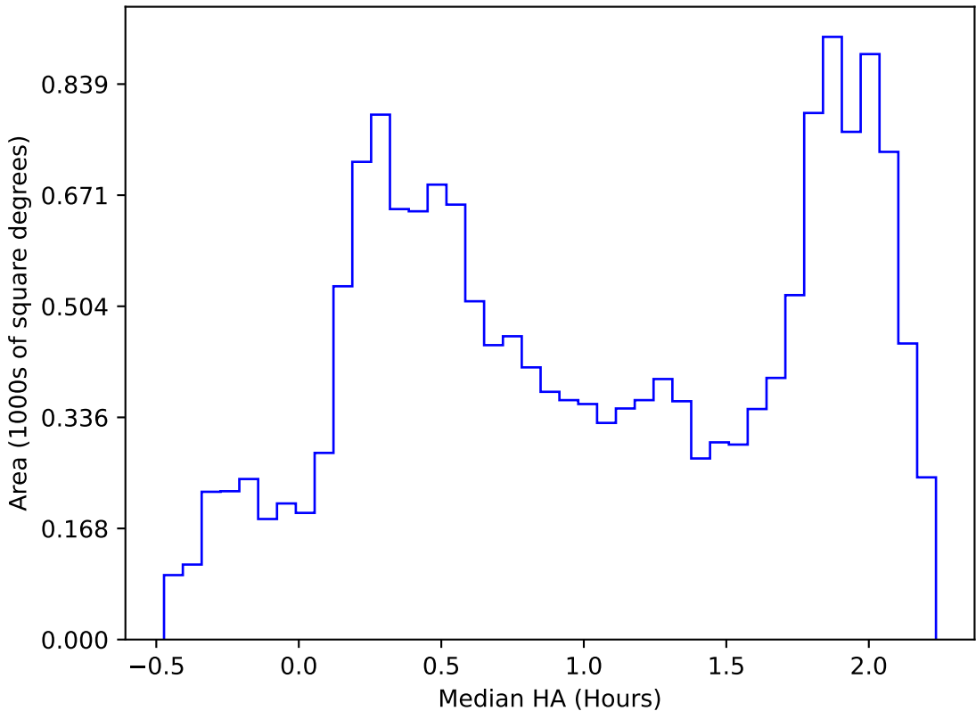
internal_u_expt38_nscale1.0v3.4_10yrs WFD all bands: Median HA
