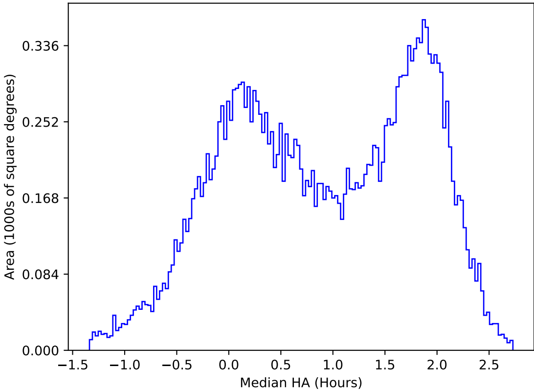
internal_u_expt38_nscale1.0v3.4_10yrs All sky u band: Median HA
