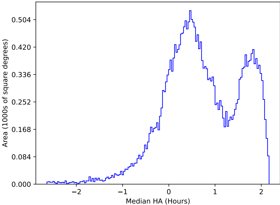
internal_u_expt38_nscale1.0v3.4_10yrs All sky r band: Median HA
