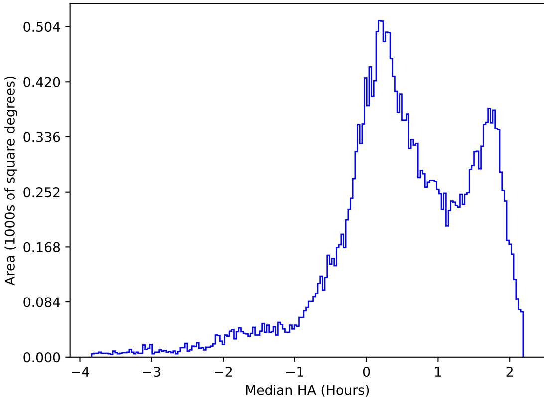
internal_u_expt38_nscale1.0v3.4_10yrs All sky g band: Median HA
