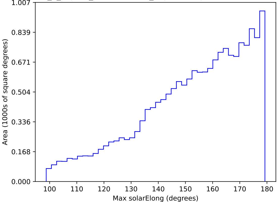
internal_u_expt38_nscale1.0v3.4_10yrs WFD y band: Max solarElong
