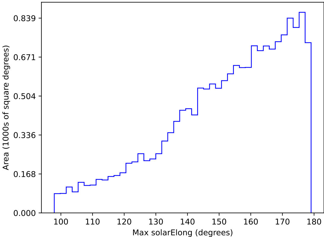
internal_u_expt38_nscale1.0v3.4_10yrs WFD u band: Max solarElong
