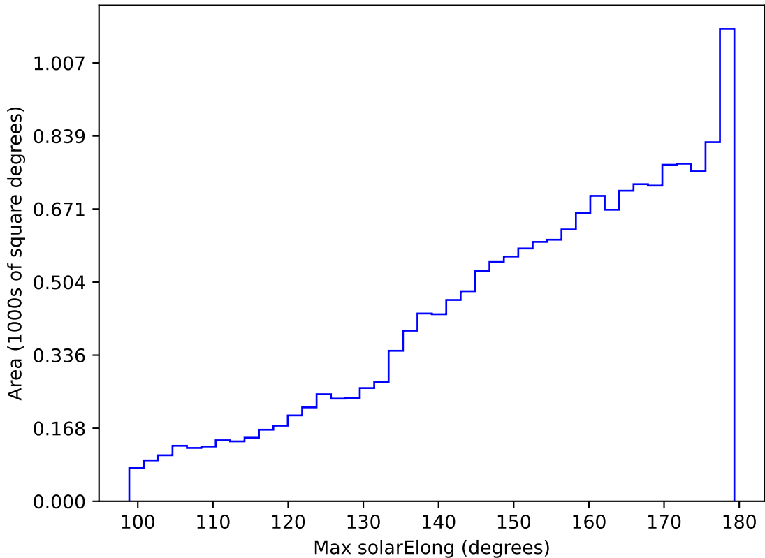
internal_u_expt38_nscale1.0v3.4_10yrs WFD i band: Max solarElong
